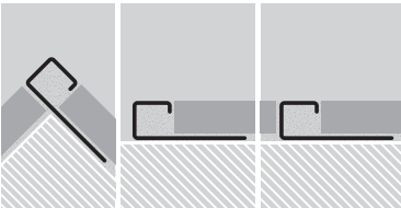
PERFIL (Largo: 2.50 m) PROFILE (Length: 8 ft 1/4 in)
