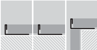
PERFIL (Largo: 2.50 m) PROFILE (Length: 8 ft 1/4 in)
